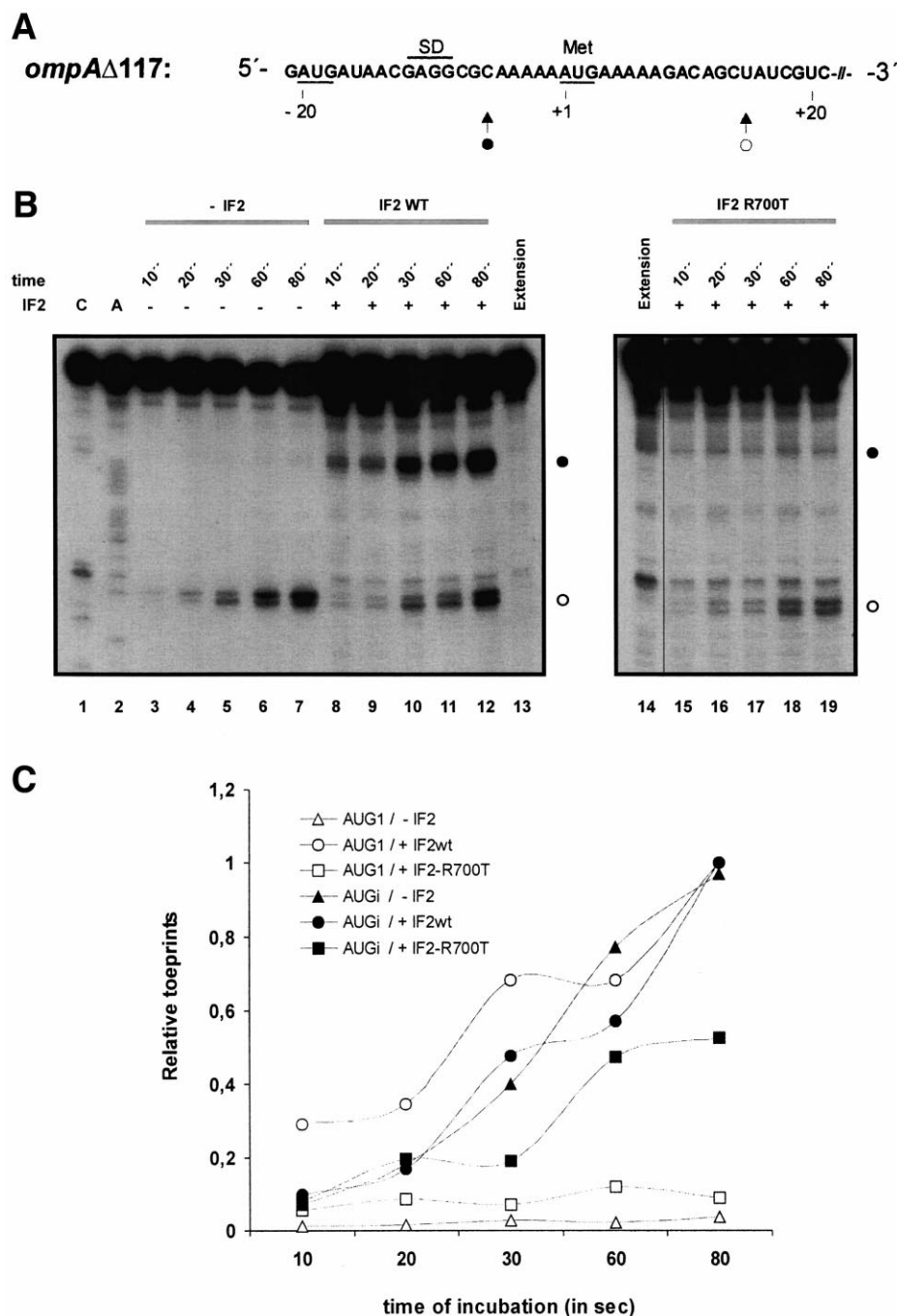
Fig. 1. Selection of the 5'-terminal (AUG1) and the internal AUG (AUGi) on ompA Δ117 mRNA in the presence of IF2 and IF2(R700T). A: Depiction of ompA Δ117 mRNA. The start codon(s) and the authentic SD sequence of ompA mRNA are indicated by bars. For ompA Δ117 two toeprinting signals are obtained, which result from ternary complex over AUG1 (nt -20–18) and AUGi (nt 1–3) the latter of which represents the authentic start codon of ompA mRNA. The positions of the toeprinting signals are indicated by a filled (AUG1) and an open circle (AUGi). B: Kinetic toeprints on ompA Δ117 mRNA in the absence or presence of IF2 and IF2(R700T), respectively. Lanes 3–7, kinetic toeprinting analysis in the absence of IF2. Lanes 8–12 and 15–19, kinetic toeprinting analysis in the presence of IF2 and IF2(R700T), respectively. Lanes 13 and 14, primer extension in the presence of fMet-tRNA Met and in the absence of 30S subunits. 30S subunits, fMet-tRNA Met , IF2 and mRNA were incubated for different times (given in s) as indicated on top. The assay conditions were as described in Section 2. The toeprinting signals obtained for AUG1 and AUGi are indicated by a filled and open circle, respectively. C: Relative toeprints on ompA Δ117 mRNA for AUG1 and AUGi. The relative toeprints at either start codon obtained in the absence of IF2 and in the presence of IF2(R700T) were normalized to that of AUG1 and AUGi obtained in the presence of IF2 after 80 s of incubation.
